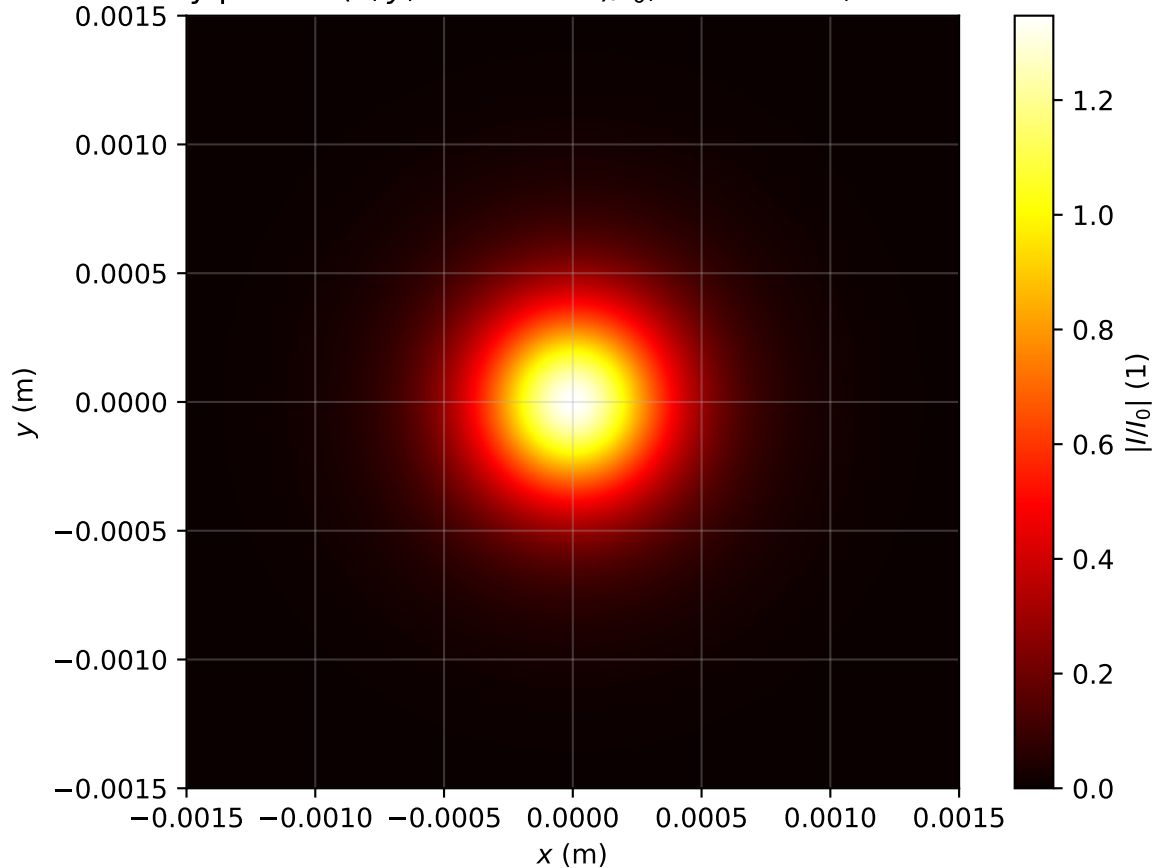
Intensity profile I(x, y, z = 1.751m)/I_0 , Pin=0.8Pcr, artificial time
